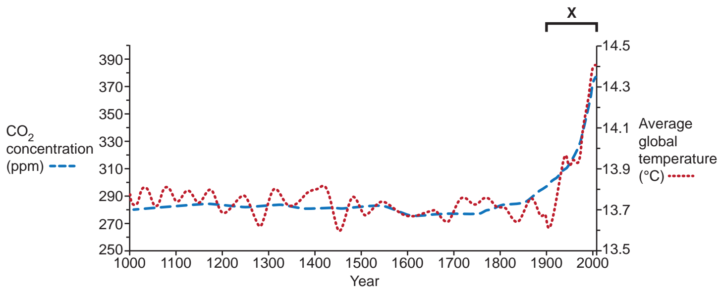
Fig. 4 Changes in global temperatures and carbon dioxide (CO 2 ) levels since 1000AD
